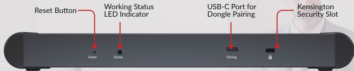
Front Panel
